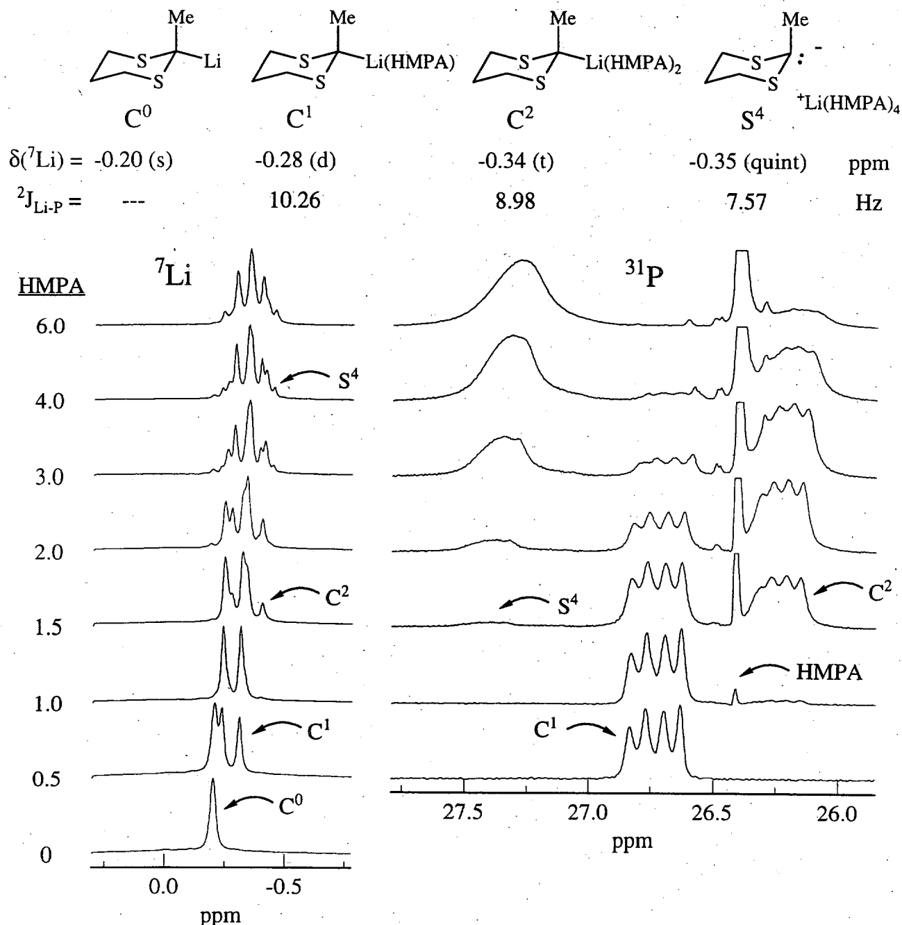
Figure S-1. ^7\text{Li} and ^{31}\text{P} NMR spectra from an HMPA titration of 0.16 M 2-methyl-1,3-dithianyllithium ( 1b-Li ) in 3:2 THF/Et 2 O at -135 °C.
